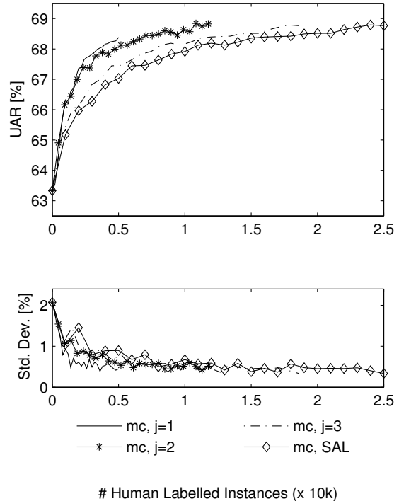
Figure 2: Dynamic Active Learning (DAL) vs Static Active Learning (SAL): the performance measures show the UAR values averaged across 20 runs of the algorithm and the respective standard deviations vs the number of human annotations.
